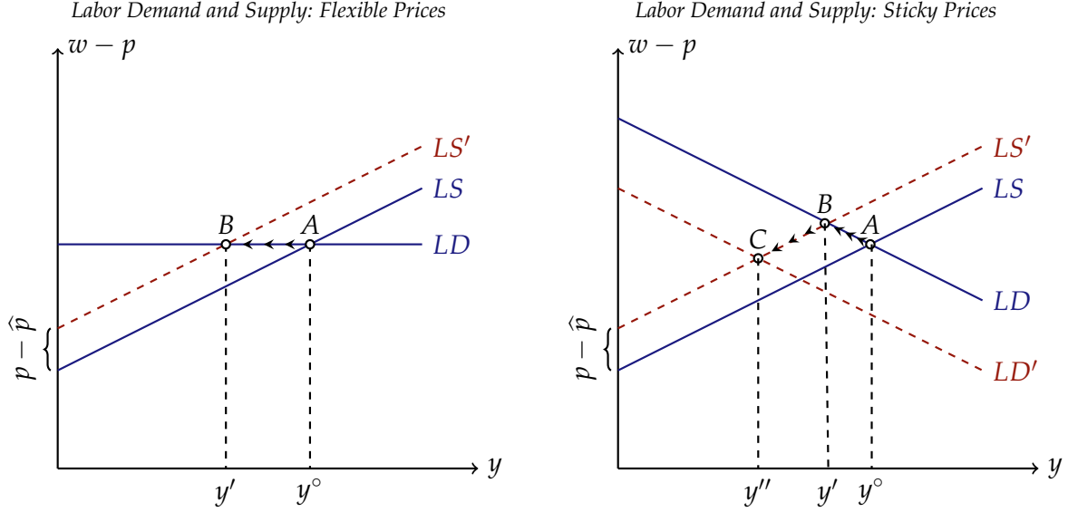
Figure 2: Interaction of LBS and price-stickiness
