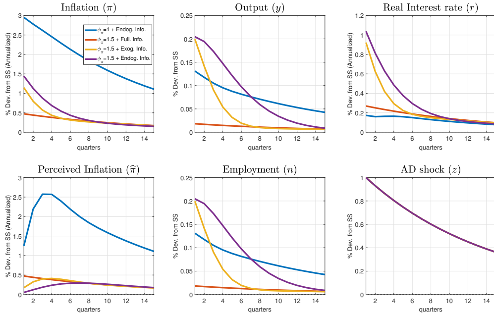
Figure 7: Dynamic Response to an Aggregate Demand Shock under Different Policy Scenarios
