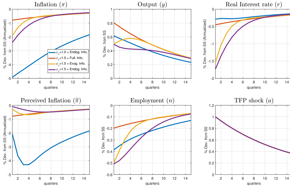
Figure 8: Dynamic Response to a Technology Shock under Different Policy Scenarios
