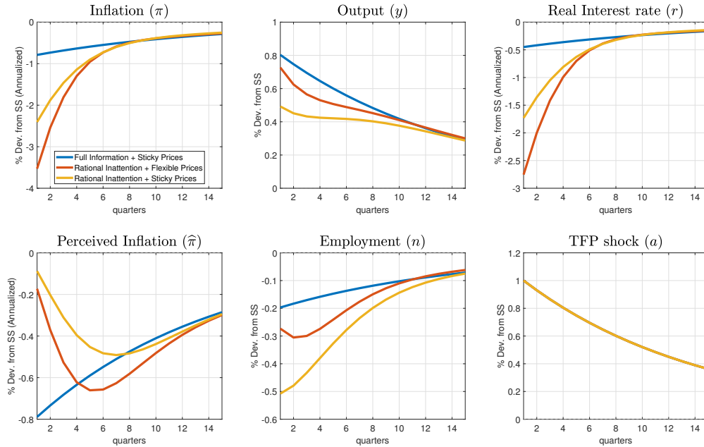
Figure 6: Dynamic Responses to a Technology Shock
