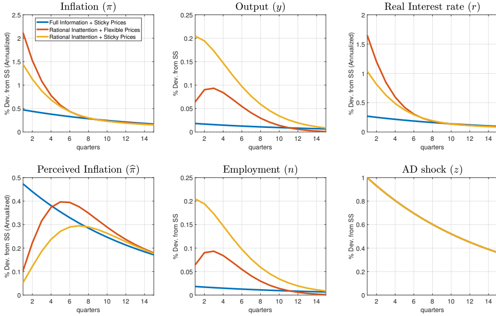
Figure 5: Dynamic Responses to an Aggregate Demand Shock
